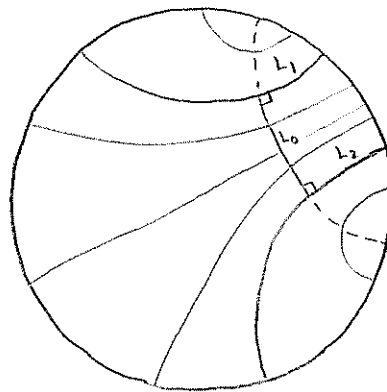
FIGURE 12. Hyperbolic pencils
