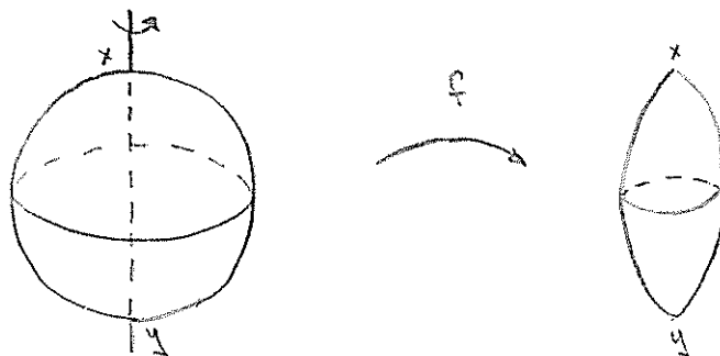
FIGURE 2. Singular points on a surface.
