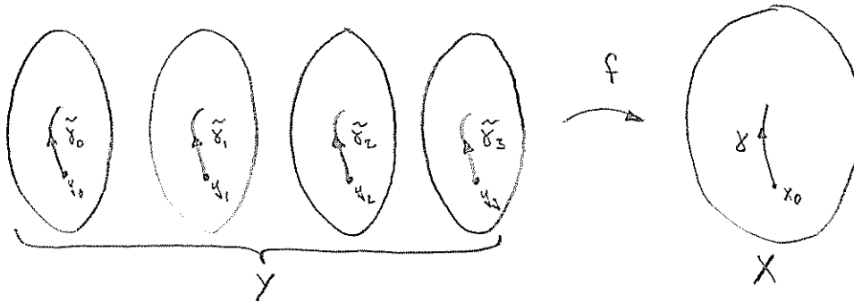
FIGURE 6. Lifts on a covering surface.
