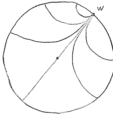
FIGURE 10. Parabolic pencils
