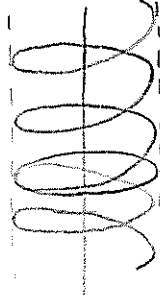
FIGURE 3. The map f from the helix to the unit circle.
