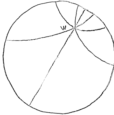
FIGURE 11. Elliptic pencils
