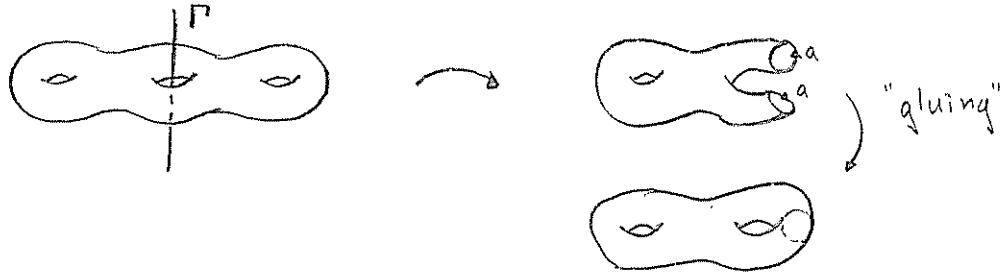
FIGURE 7. A covering of the double torus.
