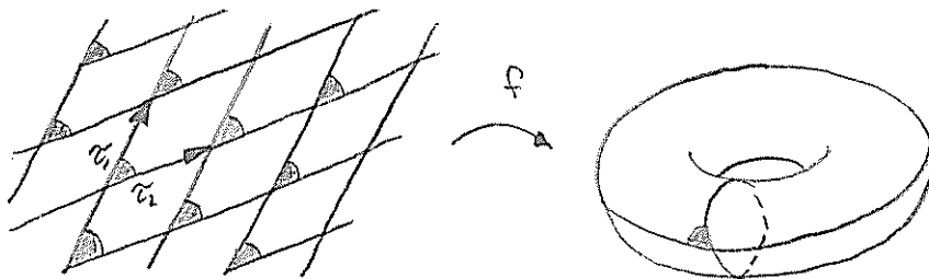
FIGURE 4. The torus as a quotient space
