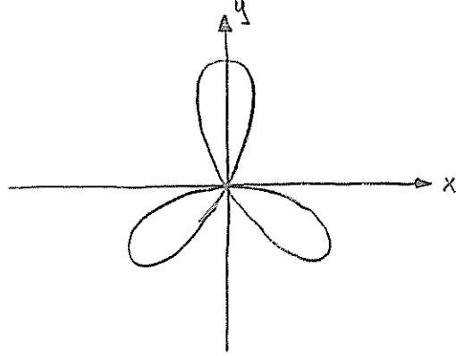
FIGURE 15. The real graph of (x^2 + y^2)^2 + 3x^2y - y^3 .
