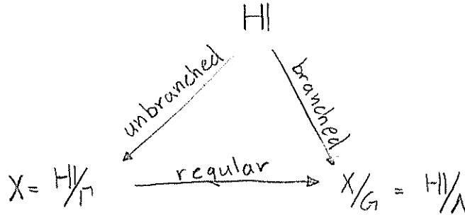
FIGURE 13. Picture of coverings
