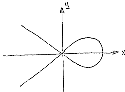
FIGURE 14. The real graph of x^3 - x^2 + y^2 .
